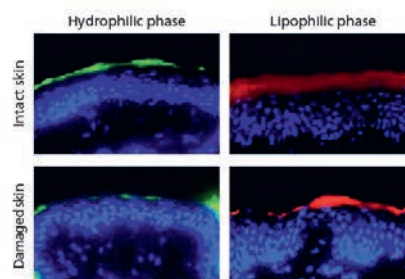
Fig. 2: Fluorescence images of the hydrophilic (green) and lipophilic phase (red) in intact and damaged skin
